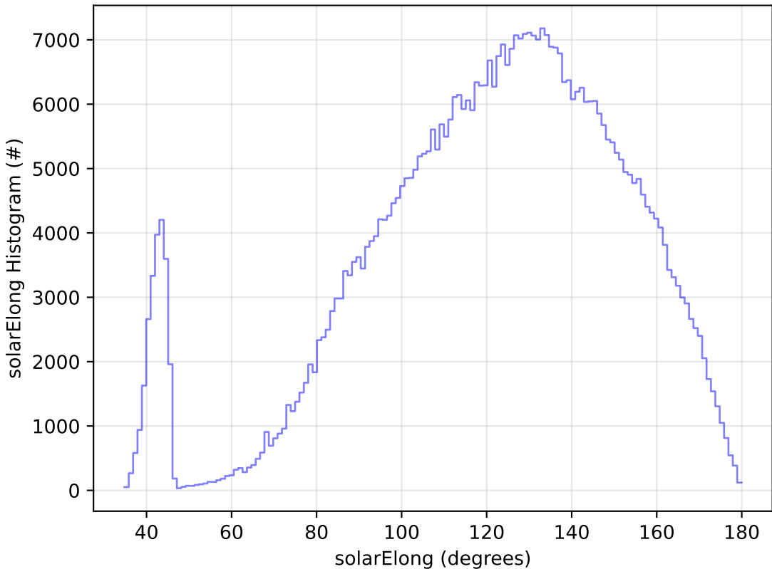
start_date_do-180v3.4_10yrs All sky i band: solarElong Histogram
