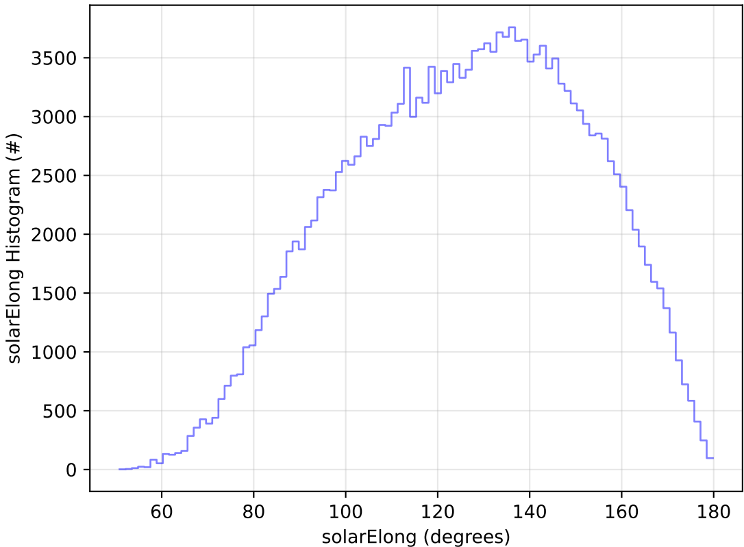
start_date_do-180v3.4_10yrs All sky g band: solarElong Histogram
