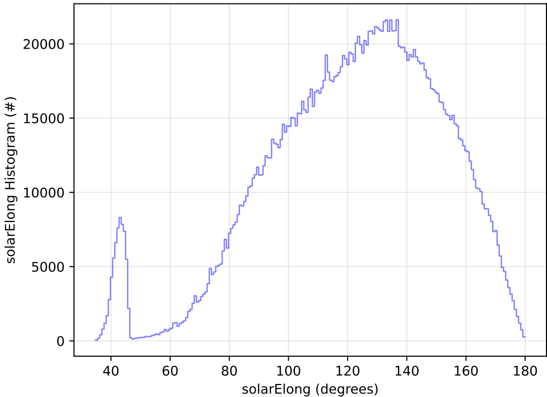
start_date_do-180v3.4_10yrs All sky all bands: solarElong Histogram
