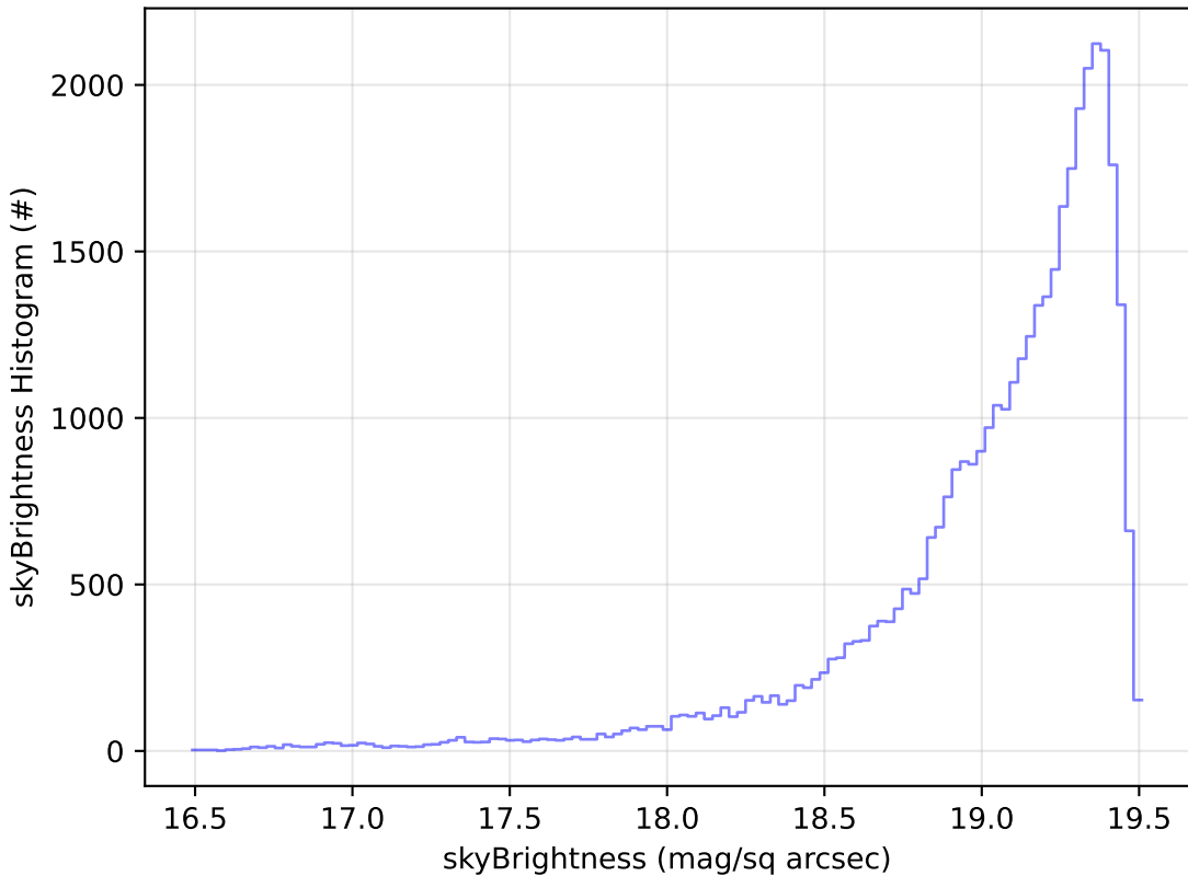
start_date_do-180v3.4_10yrs Yr 1 z band: skyBrightness Histogram
