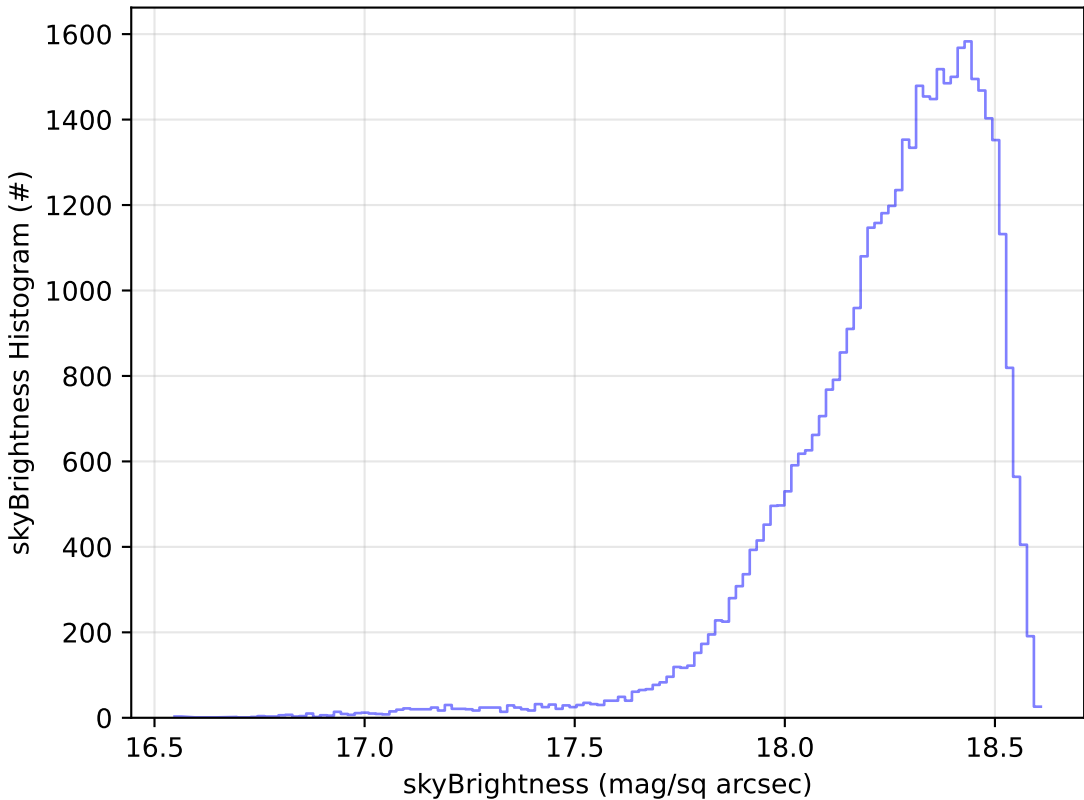
start_date_do-180v3.4_10yrs Yr 1 y band: skyBrightness Histogram
