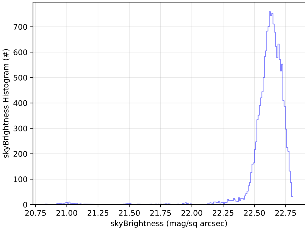
start_date_do-180v3.4_10yrs Yr 1 u band: skyBrightness Histogram
