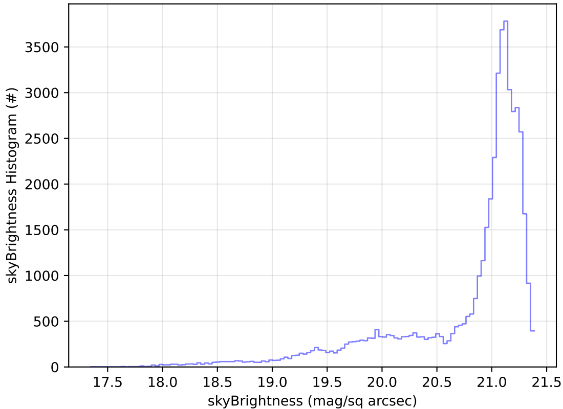
start_date_do-180v3.4_10yrs Yr 1 r band: skyBrightness Histogram
