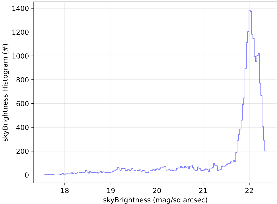
start_date_do-180v3.4_10yrs Yr 1 g band: skyBrightness Histogram
