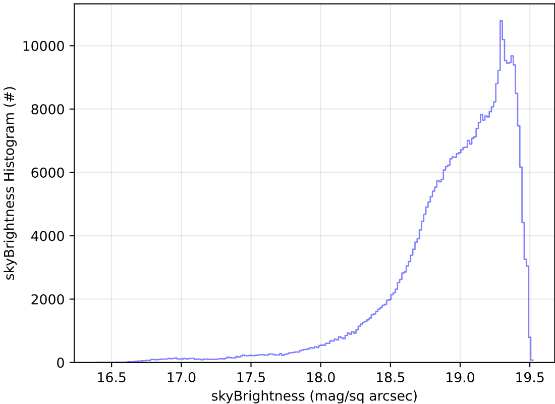
start_date_do-180v3.4_10yrs WFD z band: skyBrightness Histogram
