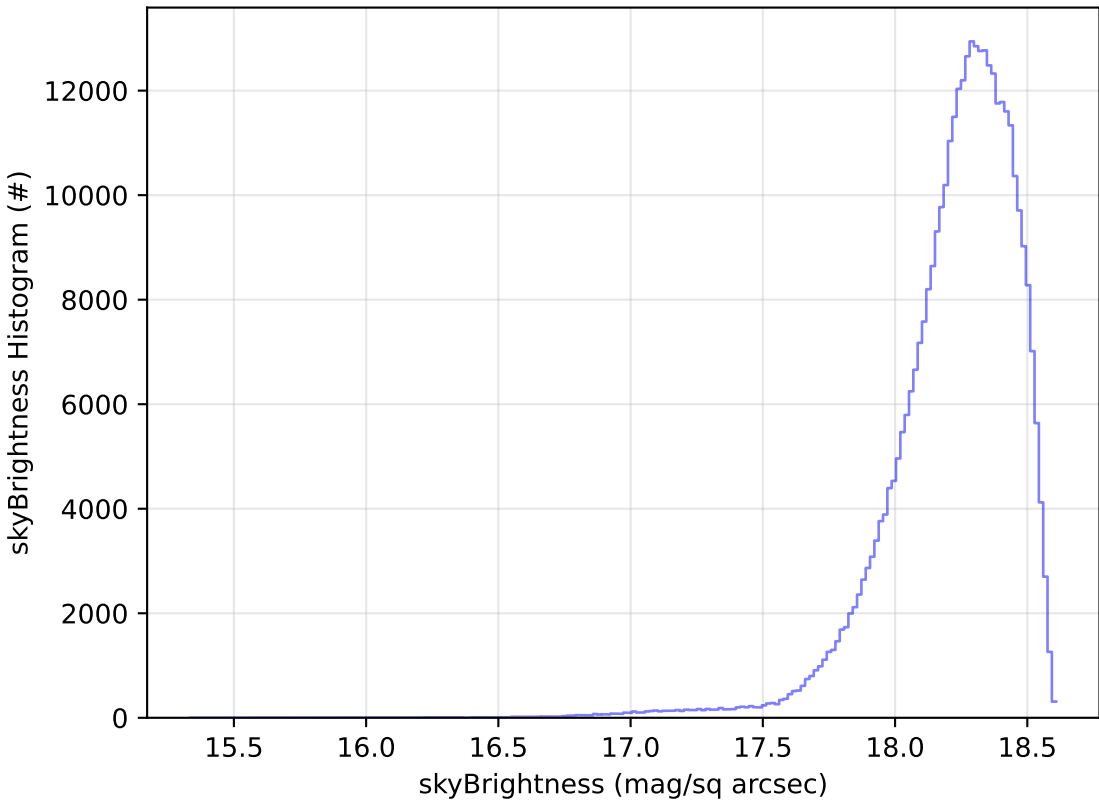
start_date_do-180v3.4_10yrs WFD y band: skyBrightness Histogram
