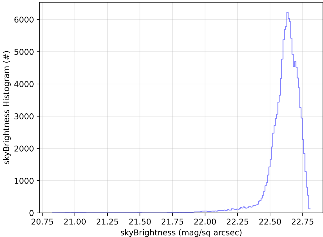
start_date_do-180v3.4_10yrs WFD u band: skyBrightness Histogram
