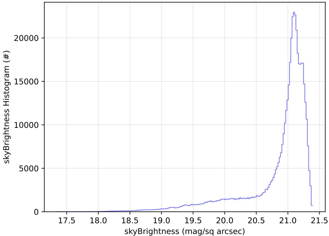
start_date_do-180v3.4_10yrs WFD r band: skyBrightness Histogram
