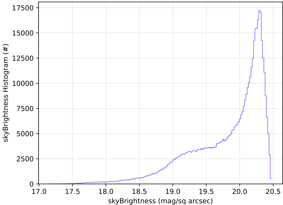
start_date_do-180v3.4_10yrs WFD i band: skyBrightness Histogram
