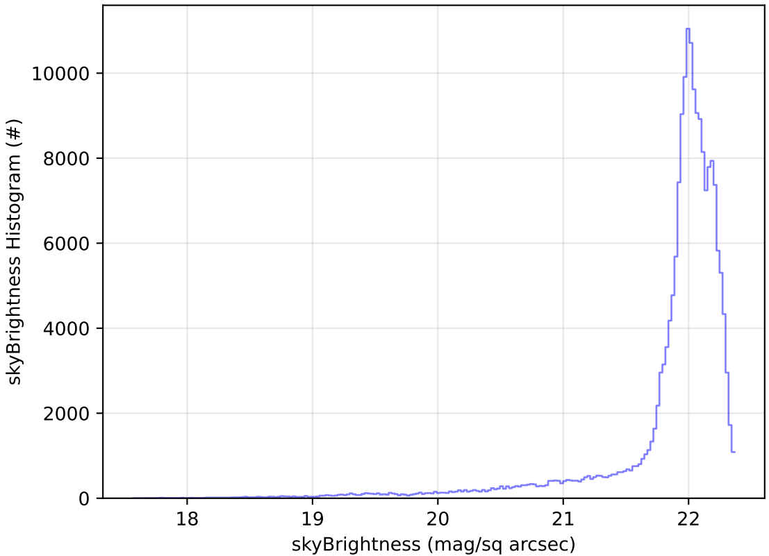
start_date_do-180v3.4_10yrs WFD g band: skyBrightness Histogram
