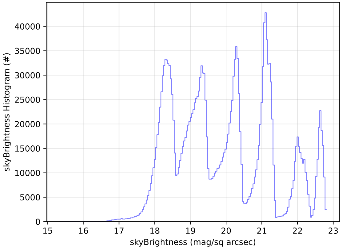
start_date_do-180v3.4_10yrs WFD all bands: skyBrightness Histogram
