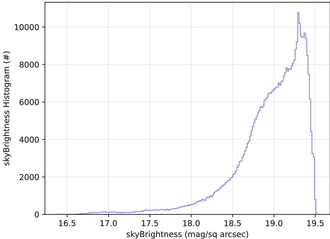
start_date_do-180v3.4_10yrs All sky z band: skyBrightness Histogram
