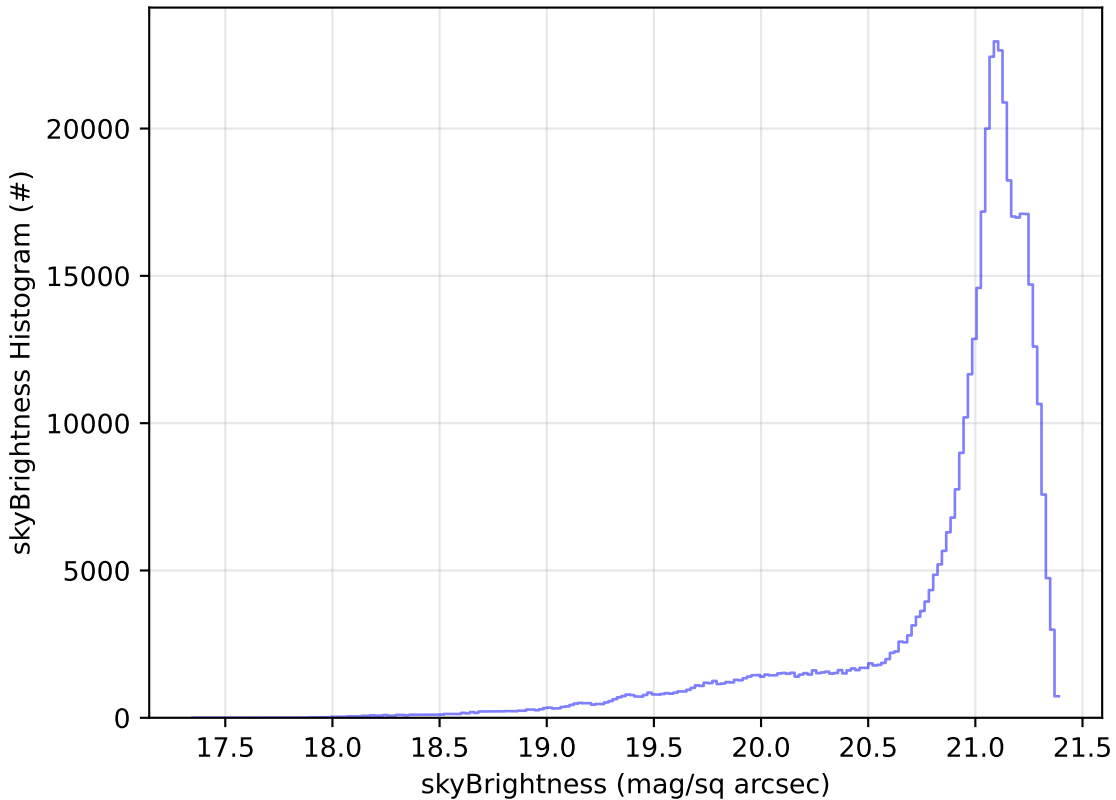
start_date_do-180v3.4_10yrs All sky r band: skyBrightness Histogram
