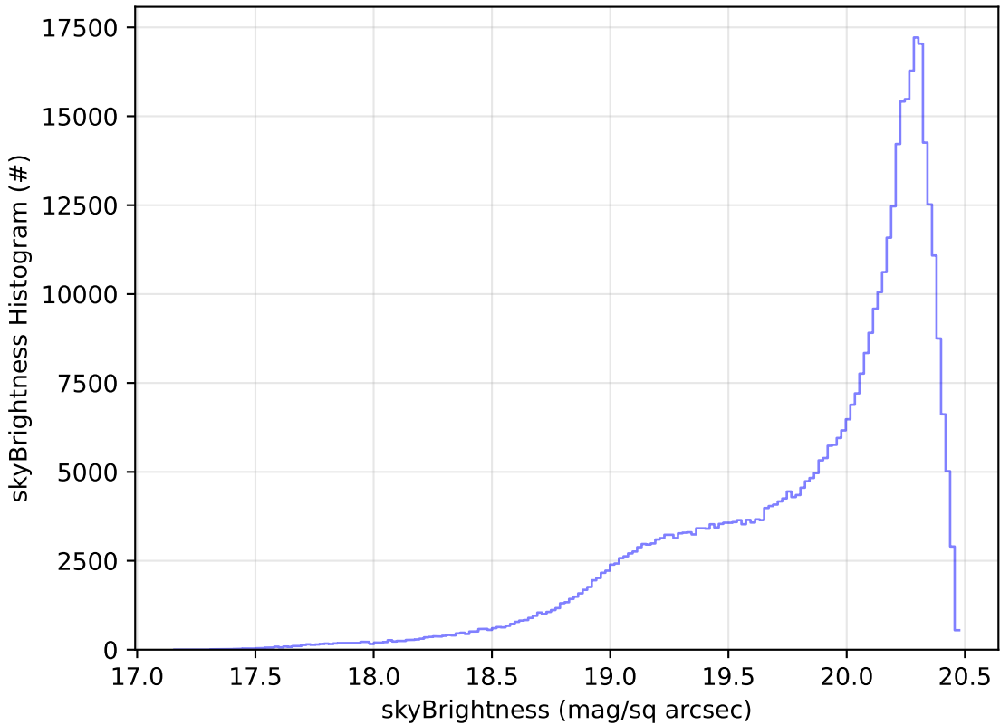
start_date_do-180v3.4_10yrs All sky i band: skyBrightness Histogram
