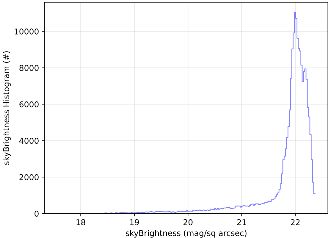
start_date_do-180v3.4_10yrs All sky g band: skyBrightness Histogram
