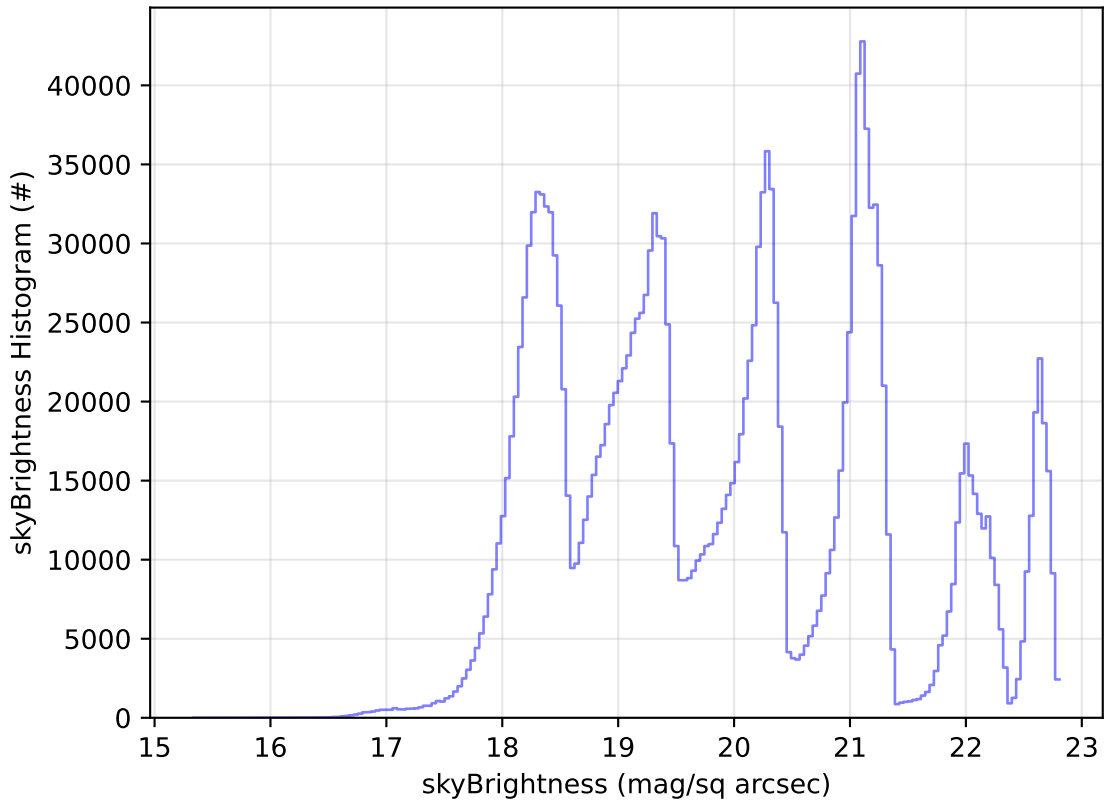
start_date_do-180v3.4_10yrs All sky all bands: skyBrightness Histogram
