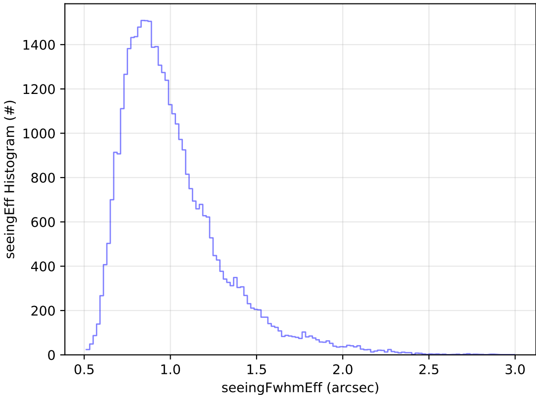
start_date_do-180v3.4_10yrs Yr 1 z band: seeingEff Histogram
