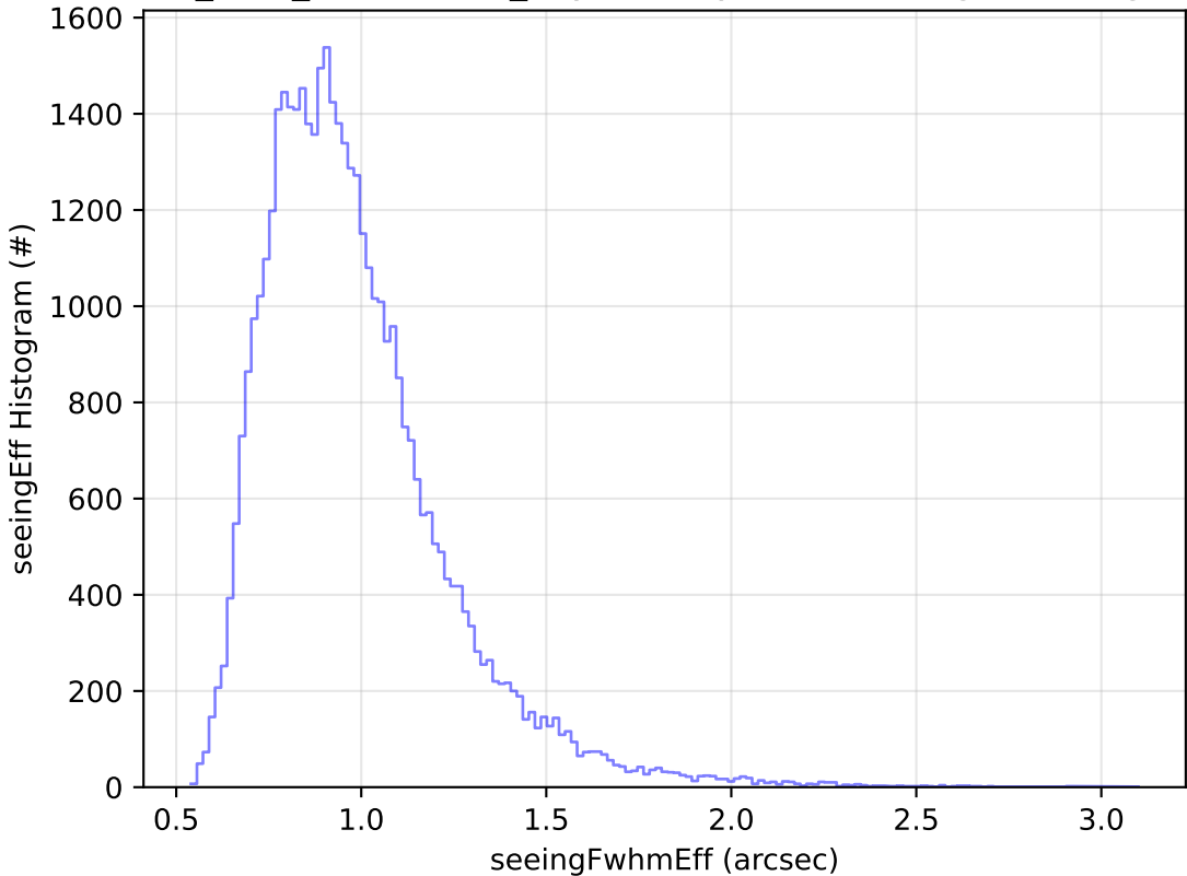
start_date_do-180v3.4_10yrs Yr 1 y band: seeingEff Histogram
