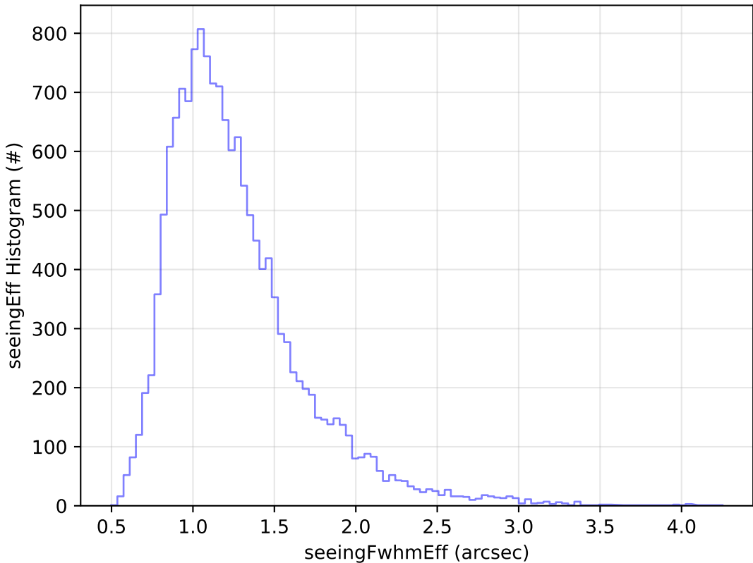
start_date_do-180v3.4_10yrs Yr 1 u band: seeingEff Histogram
