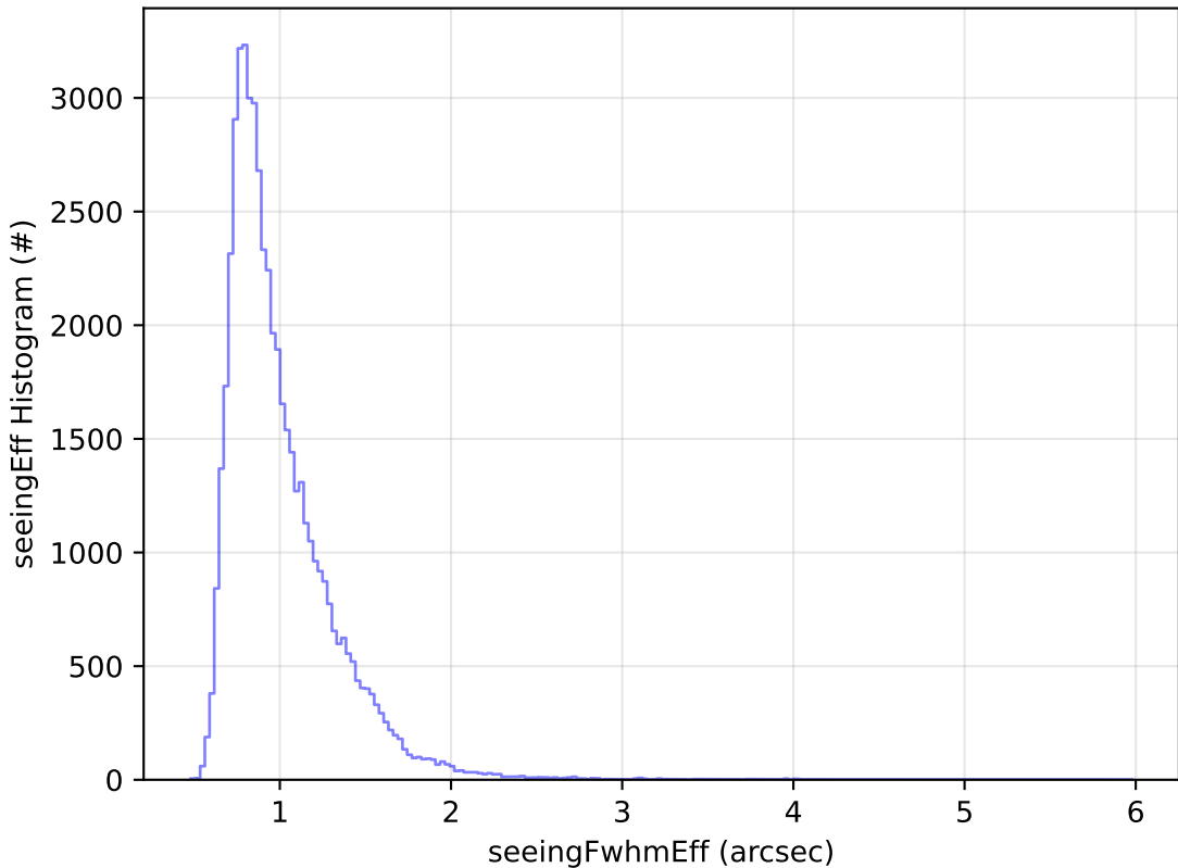
start_date_do-180v3.4_10yrs Yr 1 i band: seeingEff Histogram
