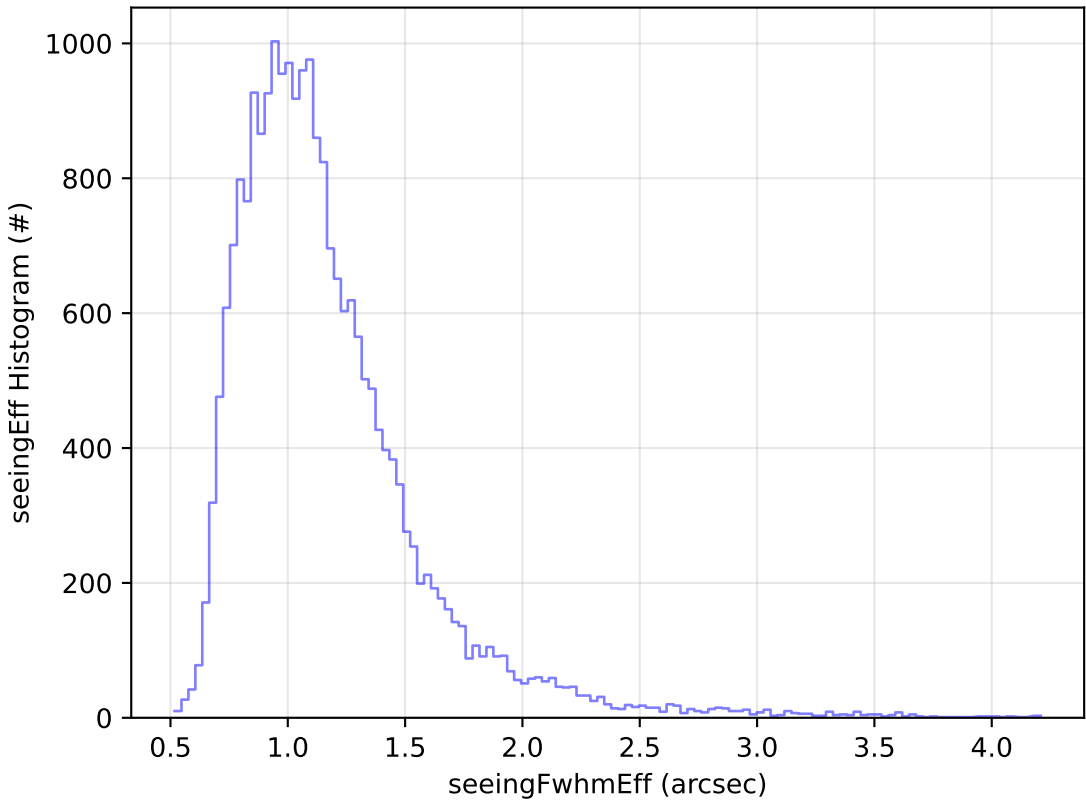
start_date_do-180v3.4_10yrs Yr 1 g band: seeingEff Histogram
