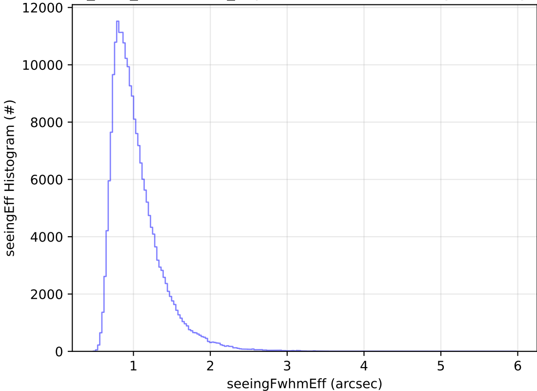
start_date_do-180v3.4_10yrs Yr 1 all bands: seeingEff Histogram
