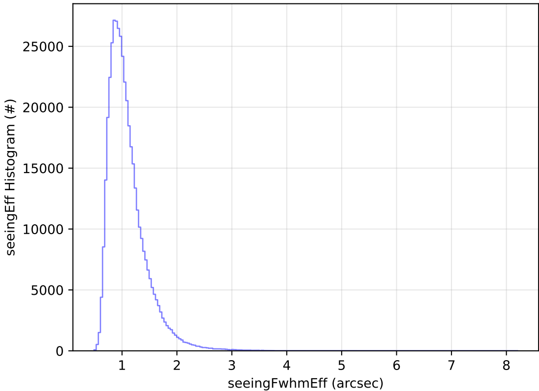
start_date_do-180v3.4_10yrs WFD z band: seeingEff Histogram
