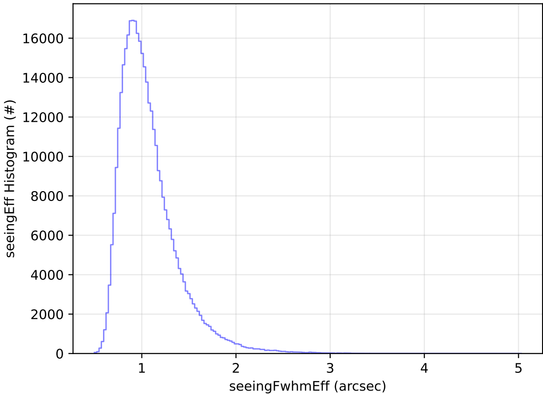
start_date_do-180v3.4_10yrs WFD y band: seeingEff Histogram
