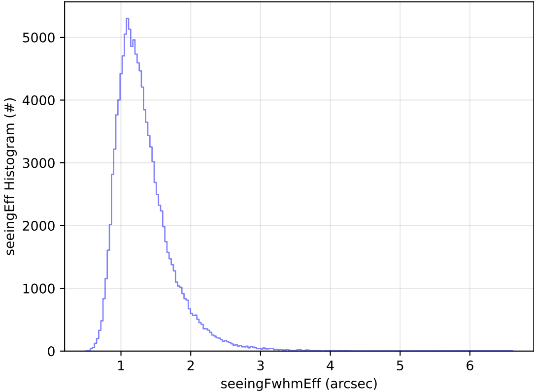
start_date_do-180v3.4_10yrs WFD u band: seeingEff Histogram
