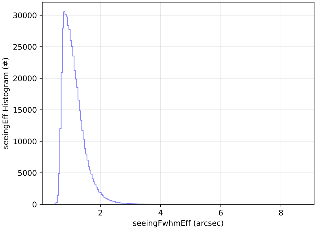
start_date_do-180v3.4_10yrs WFD r band: seeingEff Histogram
