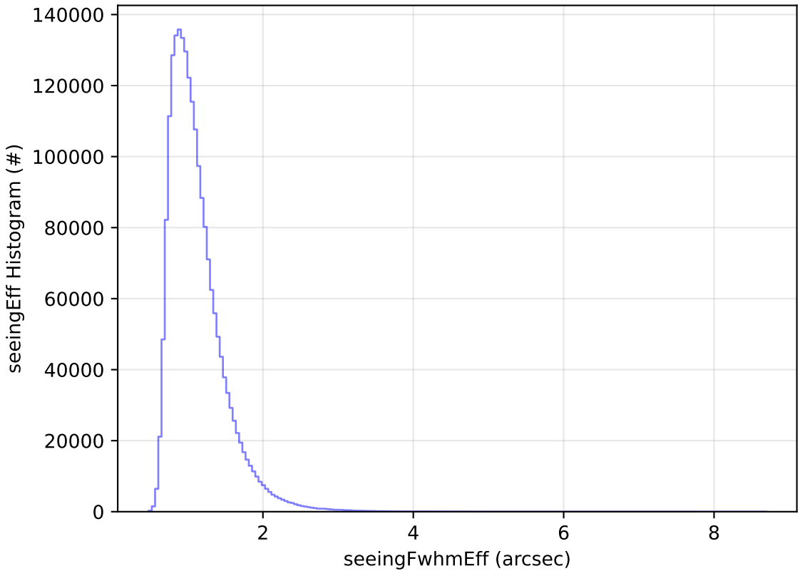
start_date_do-180v3.4_10yrs WFD all bands: seeingEff Histogram
