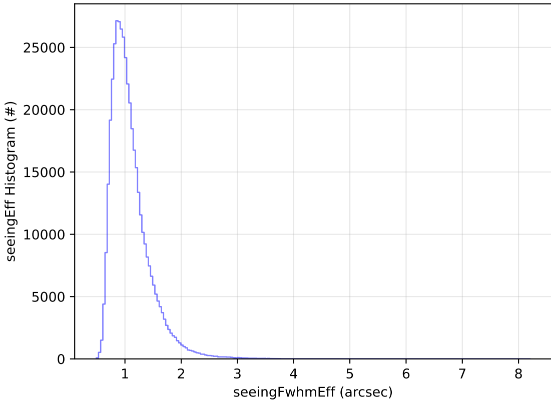
start_date_do-180v3.4_10yrs All sky z band: seeingEff Histogram
