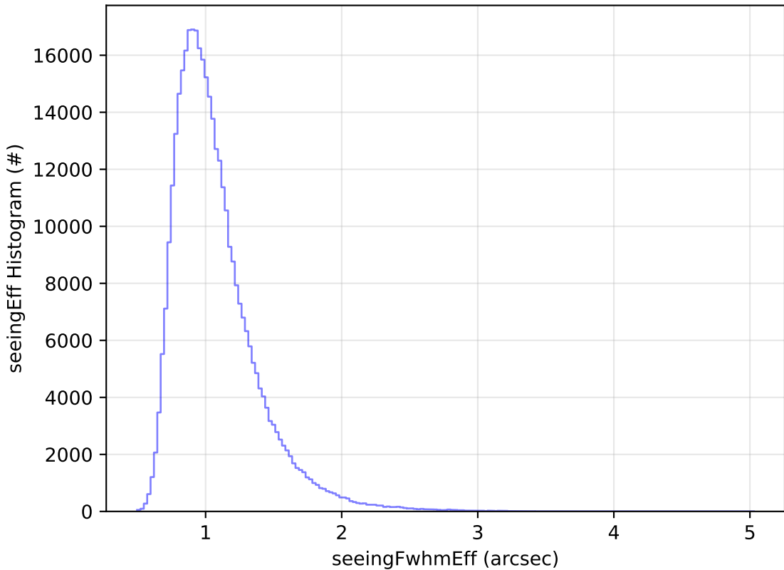
start_date_do-180v3.4_10yrs All sky y band: seeingEff Histogram
