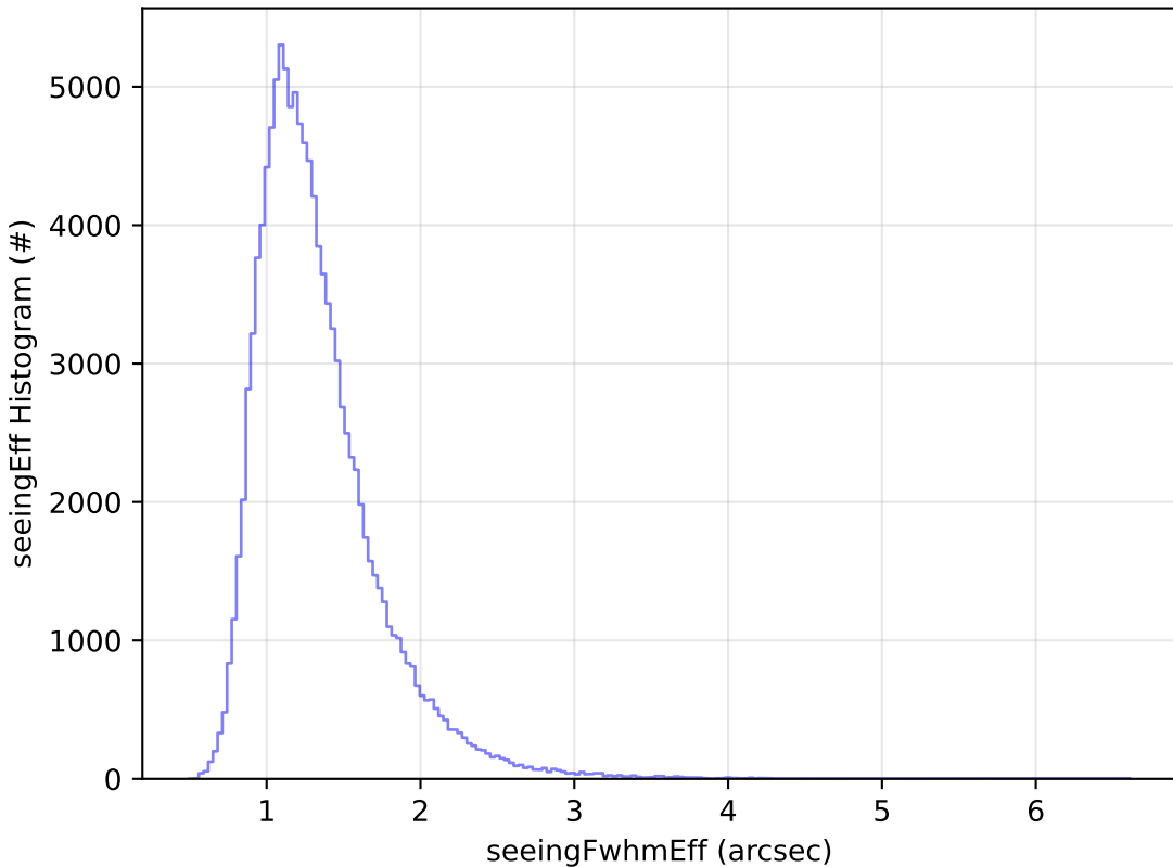
start_date_do-180v3.4_10yrs All sky u band: seeingEff Histogram
