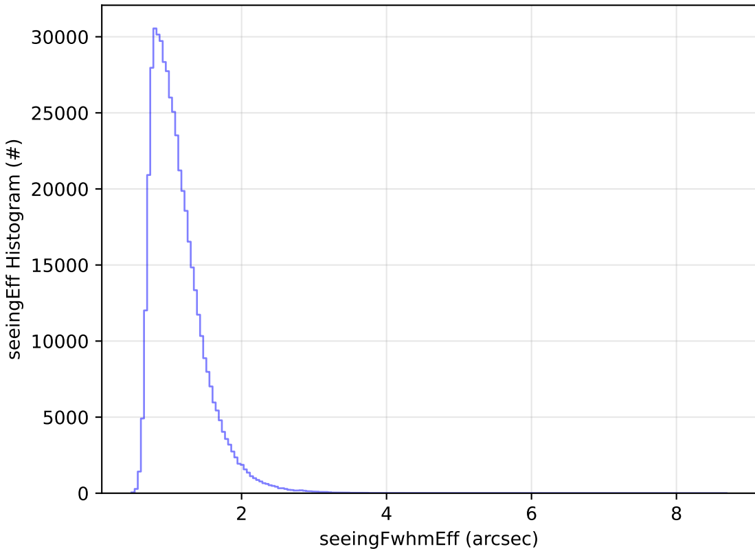
start_date_do-180v3.4_10yrs All sky r band: seeingEff Histogram
