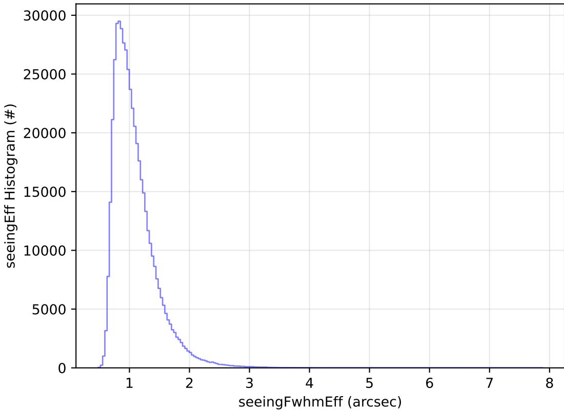
start_date_do-180v3.4_10yrs All sky i band: seeingEff Histogram
