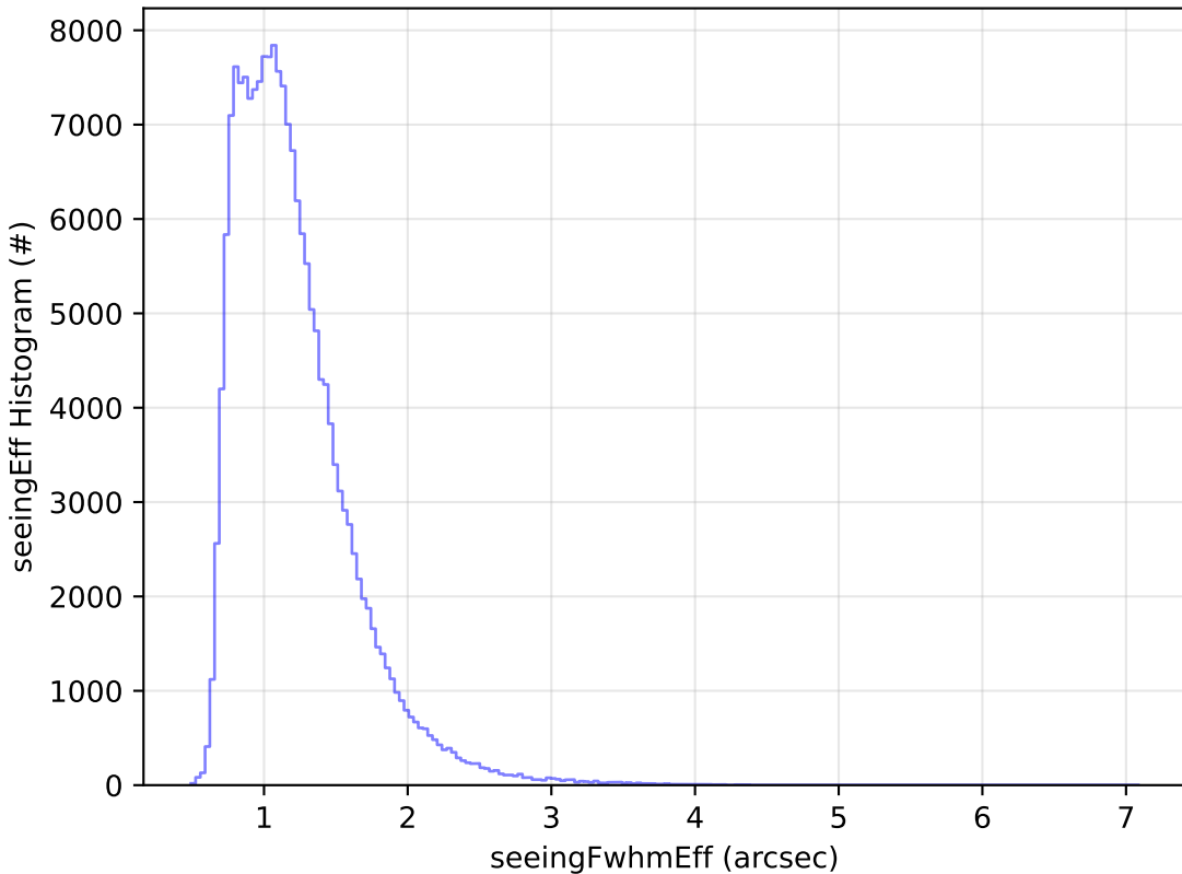
start_date_do-180v3.4_10yrs All sky g band: seeingEff Histogram
