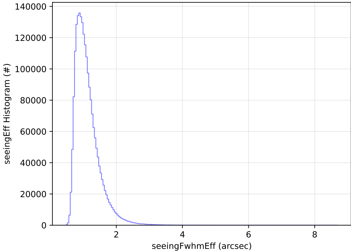
start_date_do-180v3.4_10yrs All sky all bands: seeingEff Histogram
