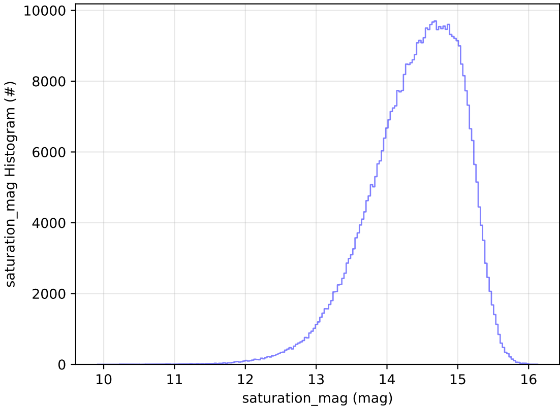
start_date_do-180v3.4_10yrs WFD i band: saturation_mag Histogram
