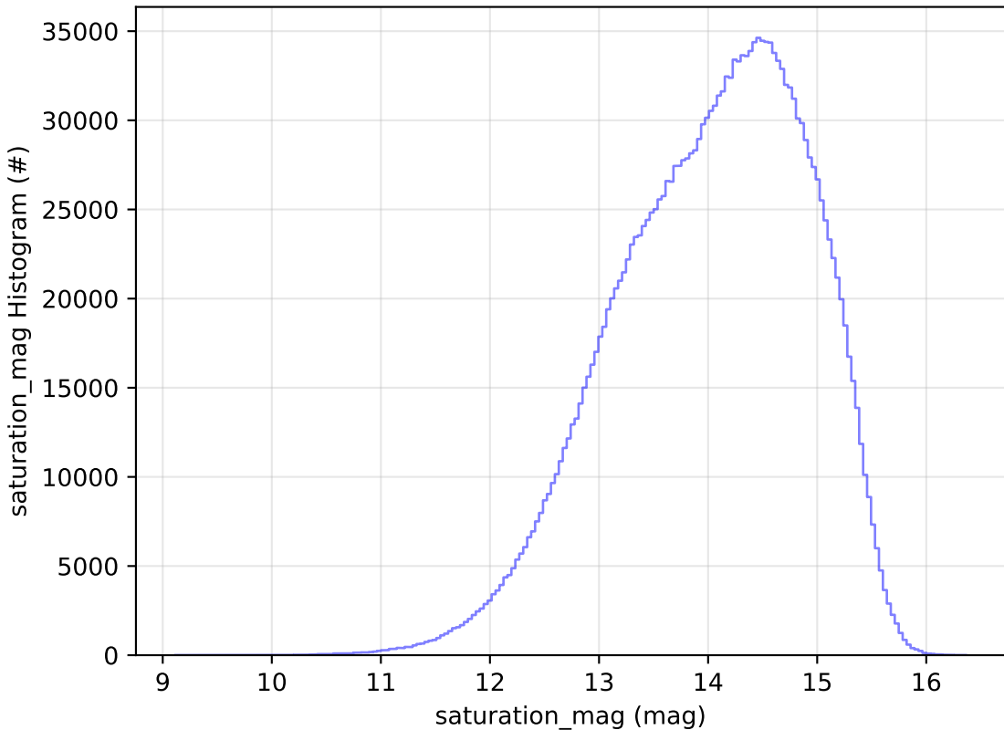
start_date_do-180v3.4_10yrs WFD all bands: saturation_mag Histogram
