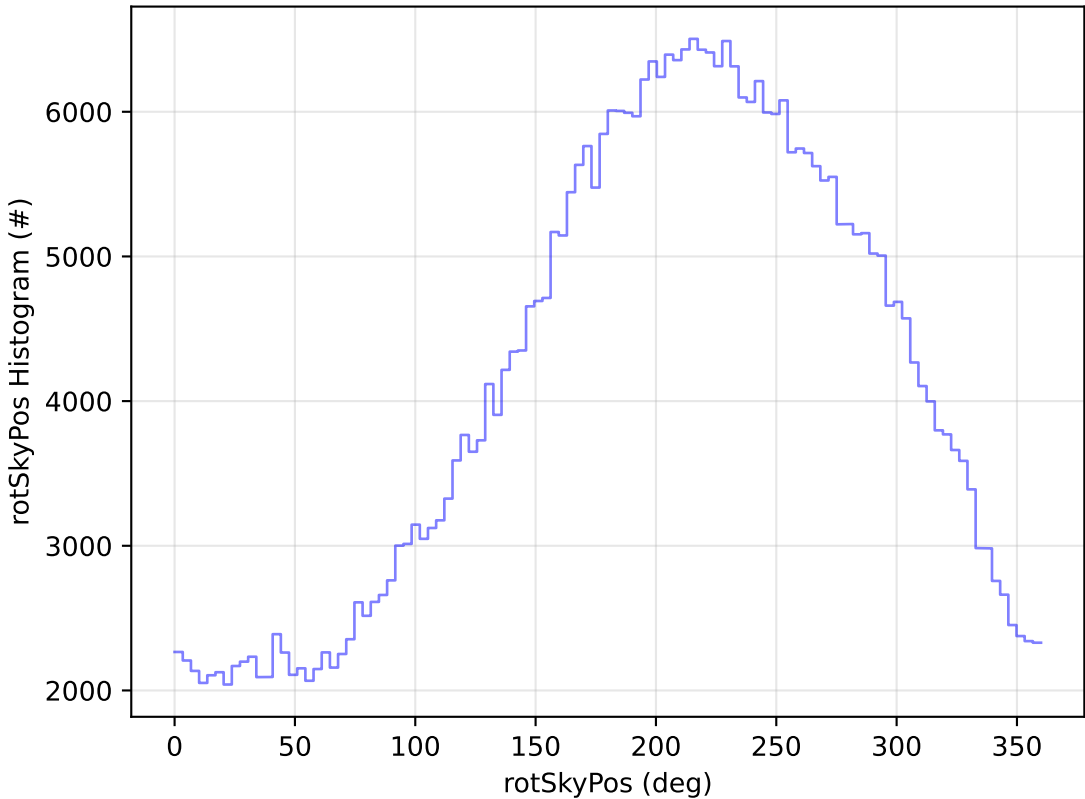
start_date_do-180v3.4_10yrs WFD z band: rotSkyPos Histogram
