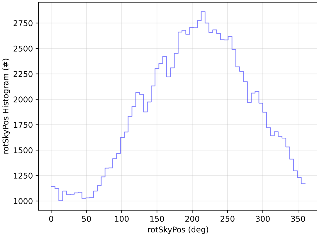
start_date_do-180v3.4_10yrs WFD u band: rotSkyPos Histogram
