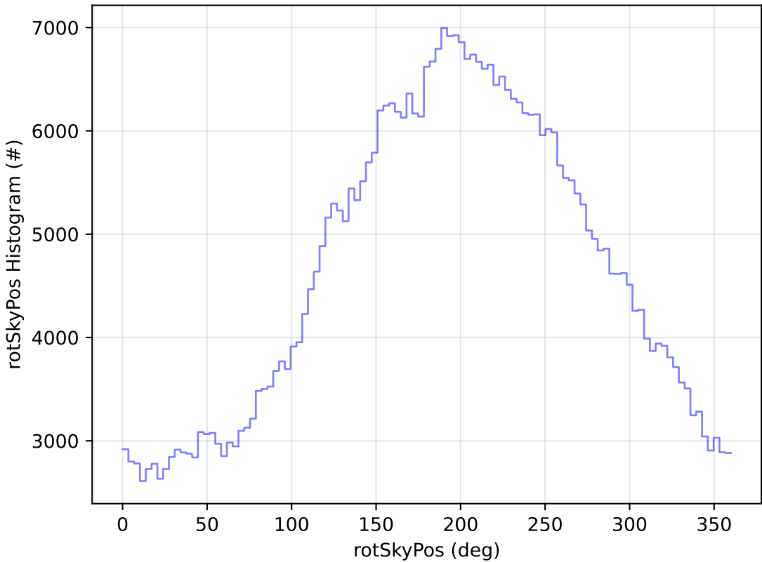
start_date_do-180v3.4_10yrs WFD r band: rotSkyPos Histogram
