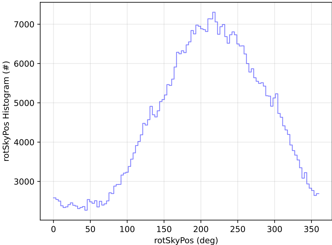
start_date_do-180v3.4_10yrs WFD i band: rotSkyPos Histogram
