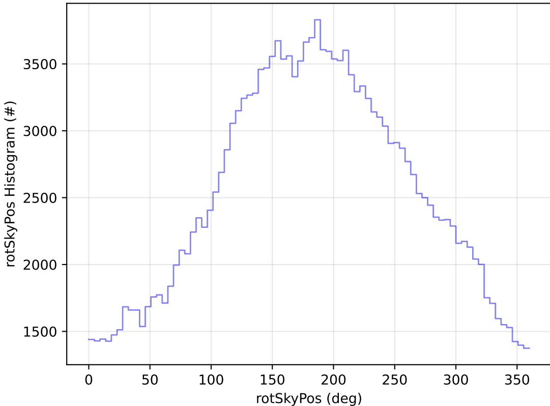
start_date_do-180v3.4_10yrs WFD g band: rotSkyPos Histogram
