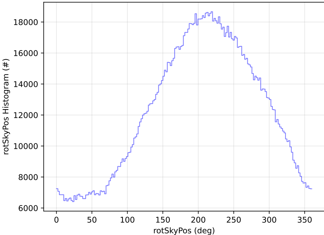
start_date_do-180v3.4_10yrs WFD all bands: rotSkyPos Histogram
