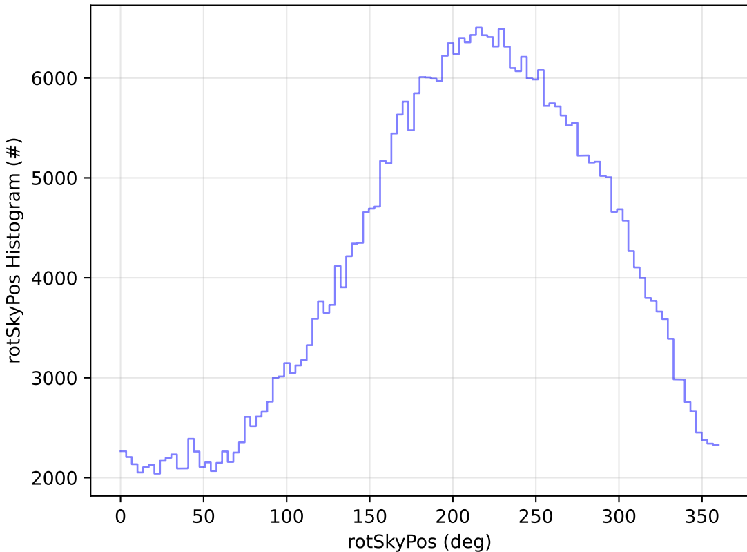
start_date_do-180v3.4_10yrs All sky z band: rotSkyPos Histogram
