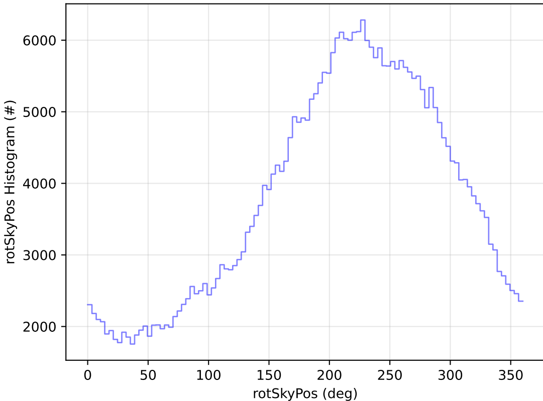
start_date_do-180v3.4_10yrs All sky y band: rotSkyPos Histogram
