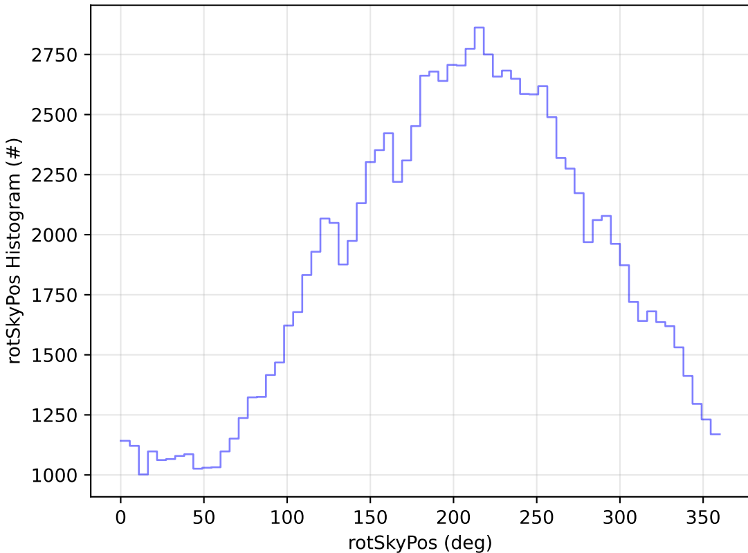
start_date_do-180v3.4_10yrs All sky u band: rotSkyPos Histogram
