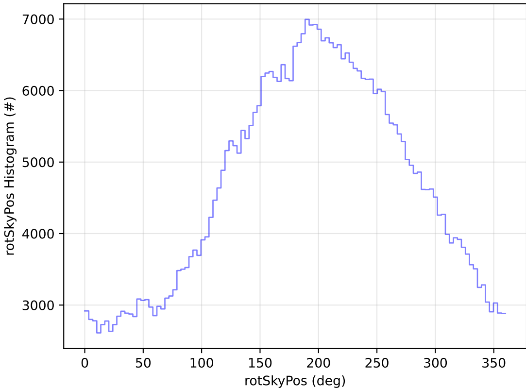
start_date_do-180v3.4_10yrs All sky r band: rotSkyPos Histogram
